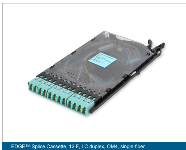
EDGE™ Splice Cassette, 12 F, LC duplex, OM4, single-fiber
